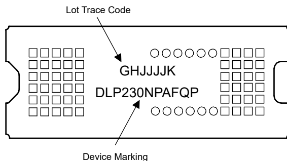
Figure 10-2. DMD Marking
