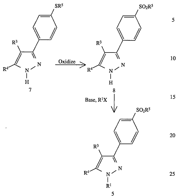
Scheme IV
