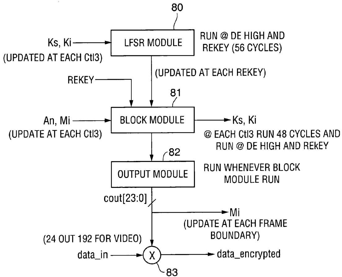
FIG. 3 (PRIOR ART)
