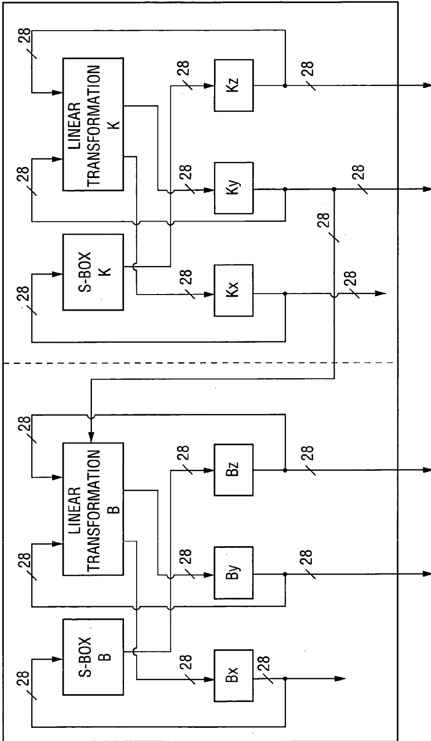
FIG. 4 (PRIOR ART)
