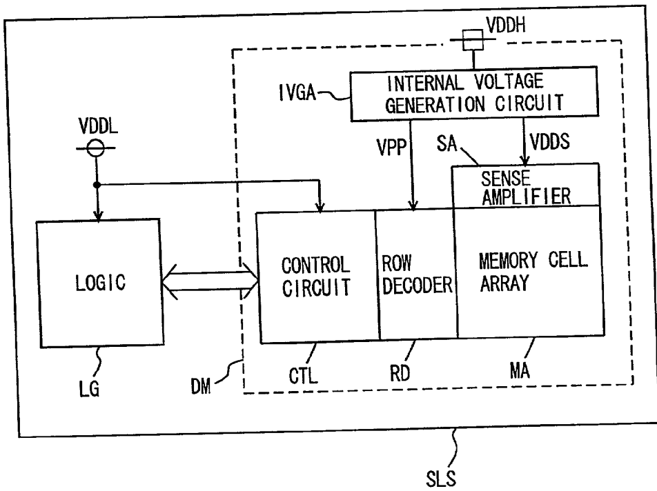
FIG. 17 PRIOR ART
