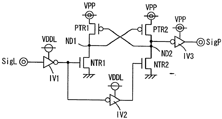
FIG. 18 PRIOR ART
