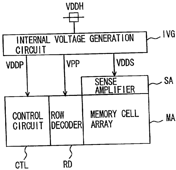
FIG. 16 PRIOR ART
