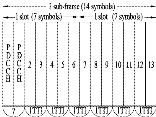
(a) 2 symbol TTI DL structure
