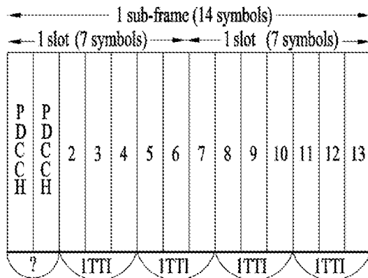
(b) 3 symbol TTI DL structure
