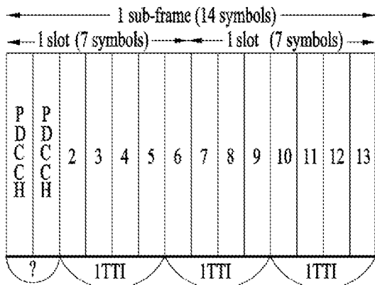
(c) 4 symbol TTI DL structure
