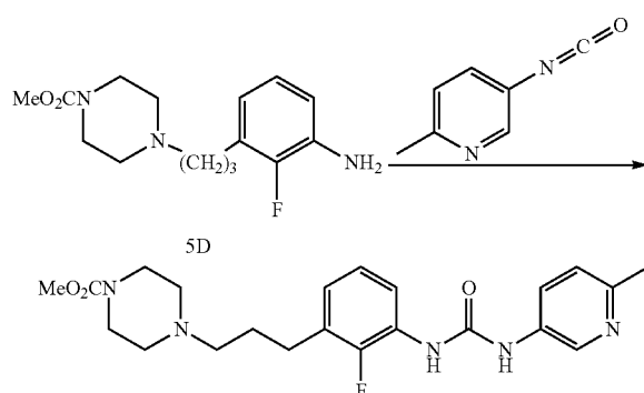
methyl 4-(3-(2-fluoro-3-(3-(6-methylpyridin-3-yl)ureido)phenyl)propyl)piperazine-1-carboxylate
