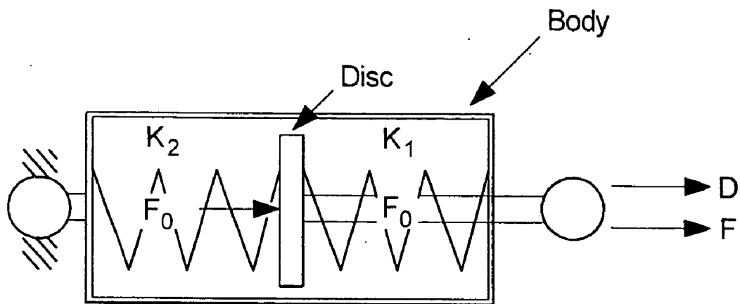
Free-body diagram
