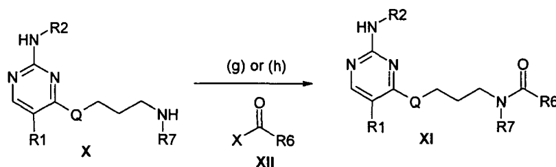
Scheme 4
