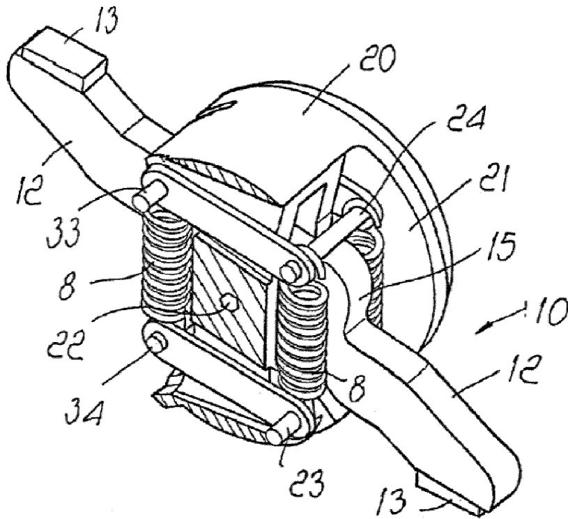
Fig. 1c (Prior art)
