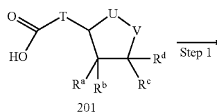
Reaction Scheme 2
