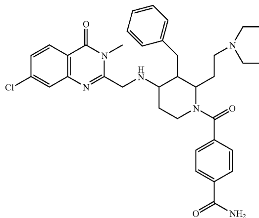
Formula IID
