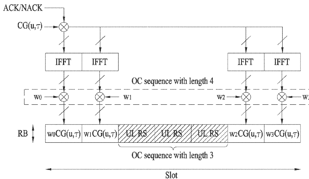
PUCCH format 1a/1b structure (normal CP)
