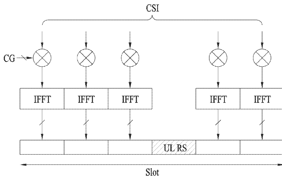
PUCCH format 2/2a/2b structure (extended CP)
