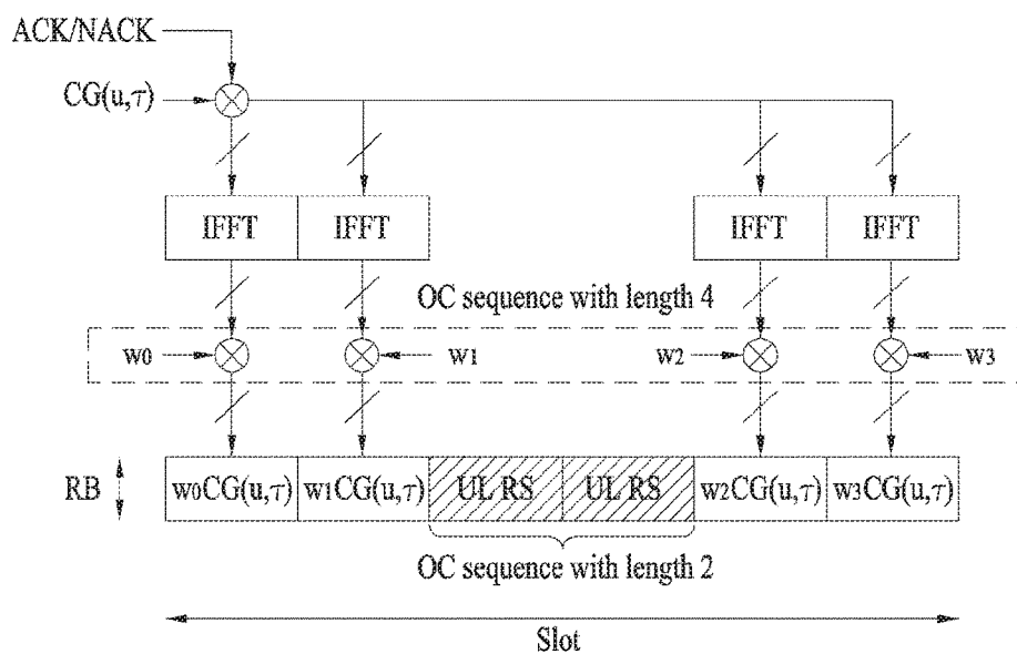
PUCCH format 1a/1b structure (extended CP)
