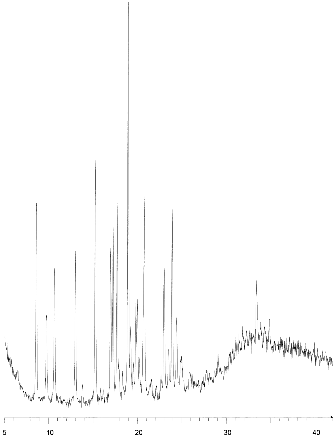
Figure 2. Compound 1 pattern 3 XRPD diffractogram
