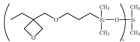
Exemplified compound 2
