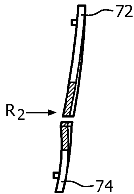
Section U-U FIG. 14C
