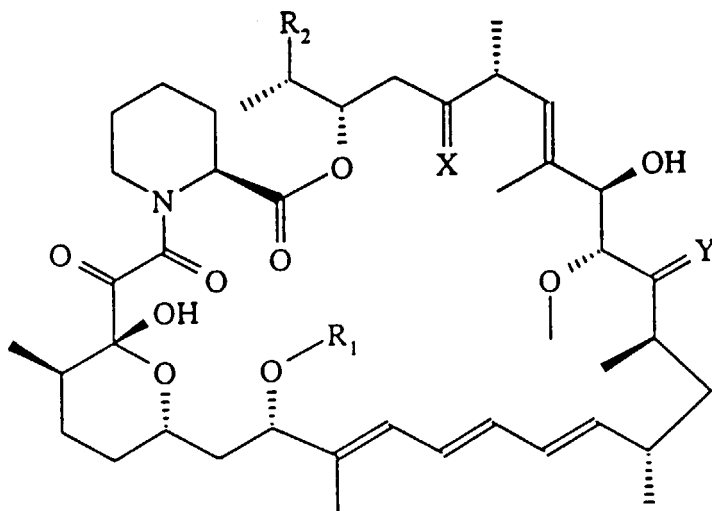
Formel I
