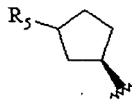
Formula III
