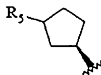
Formel III
