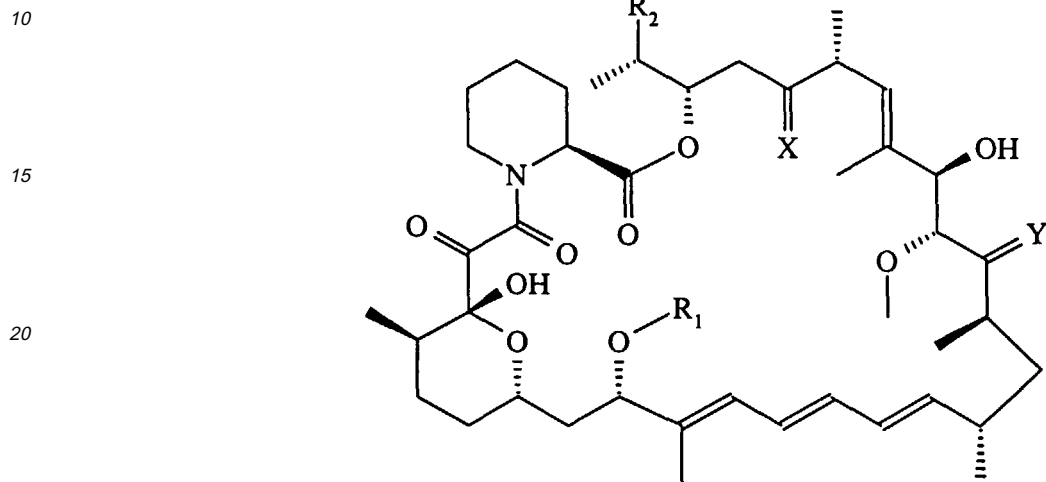
Formula I
