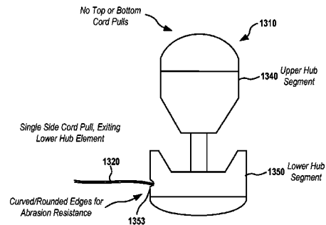
Example Embodiment of Alternate Side-Pull Hub
