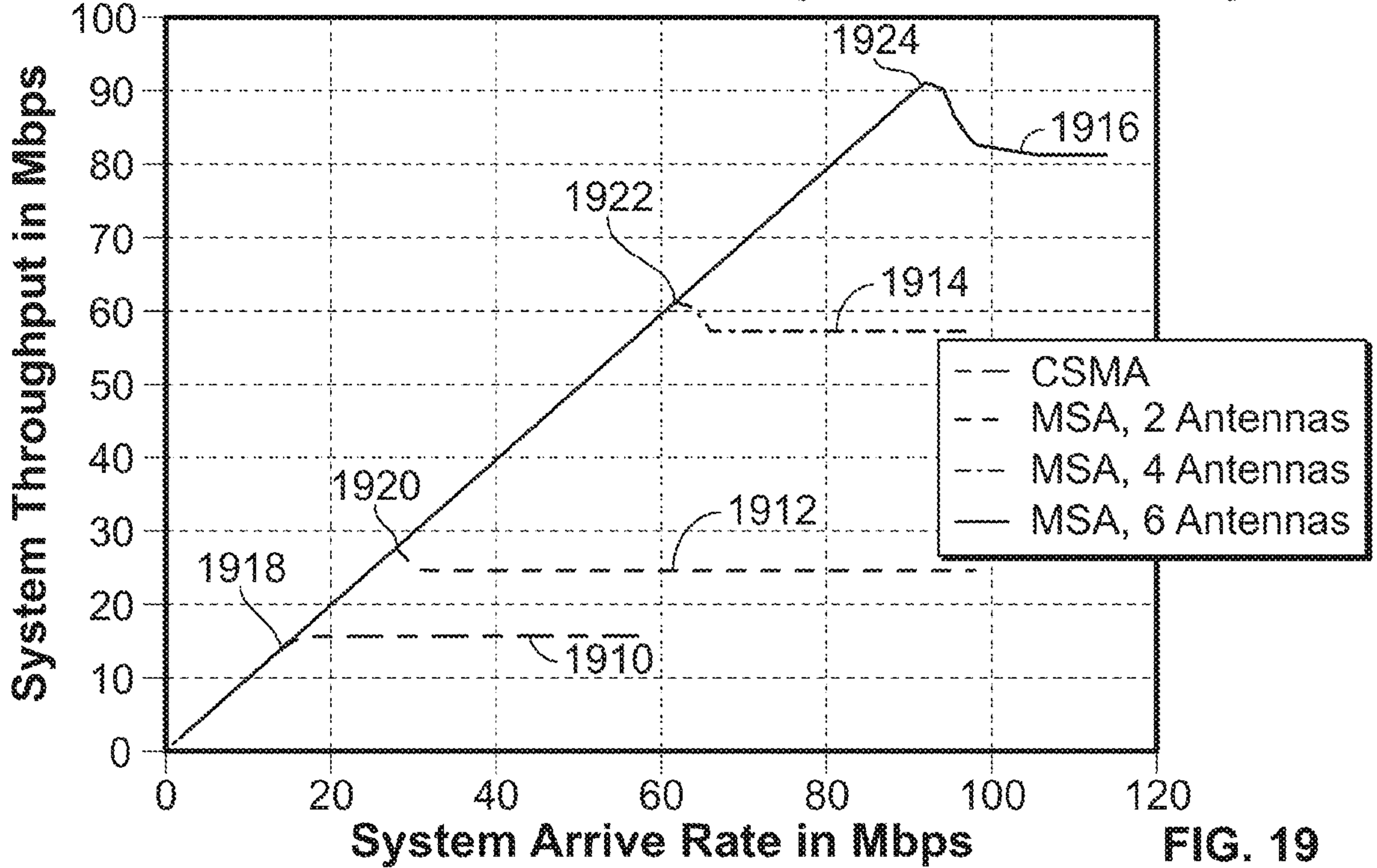
CSMA and MSA, with 13 OFDMs per Packet at 54Mbps
