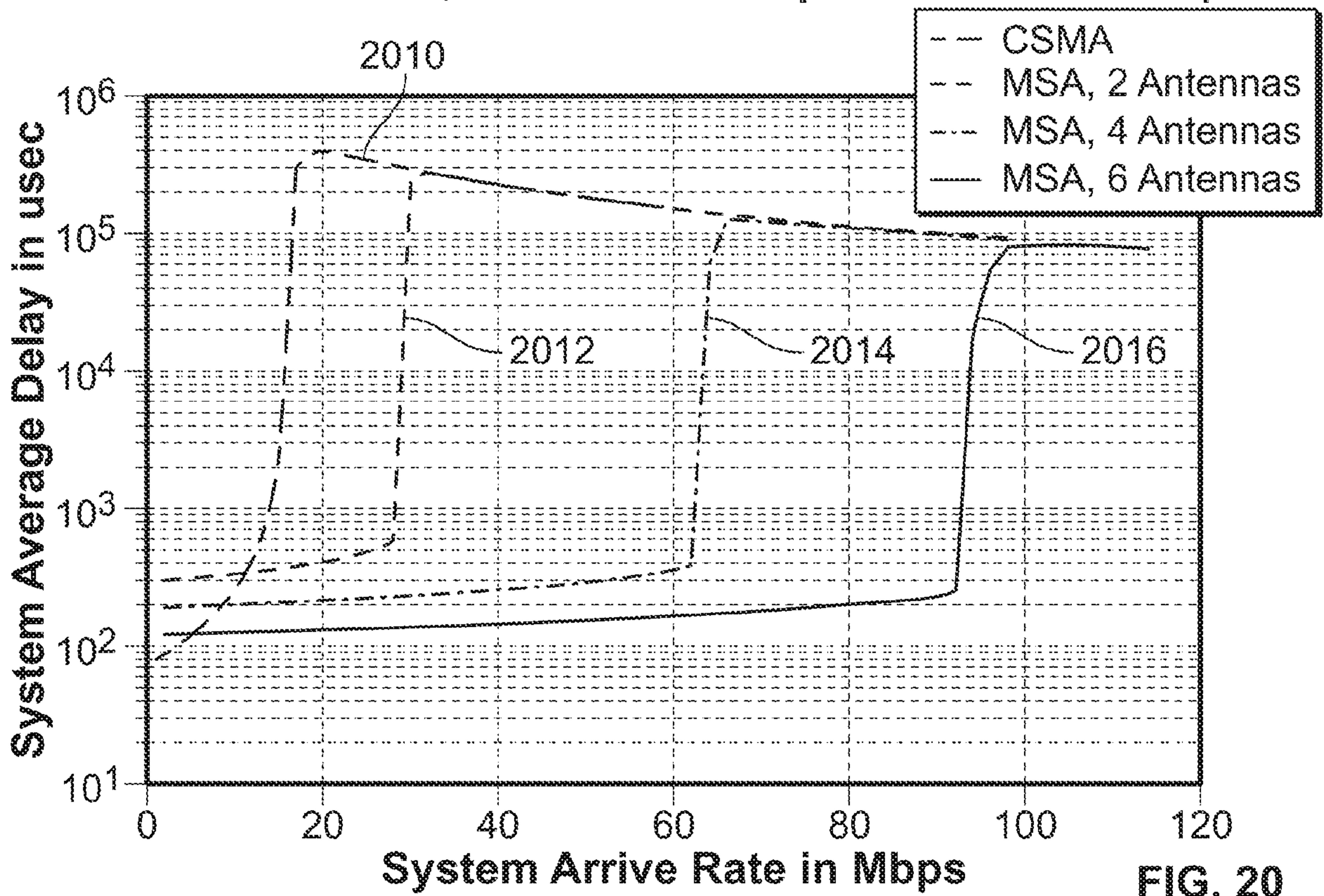
CSMA and MSA, with 13 OFDMs per Packet at 54Mbps
