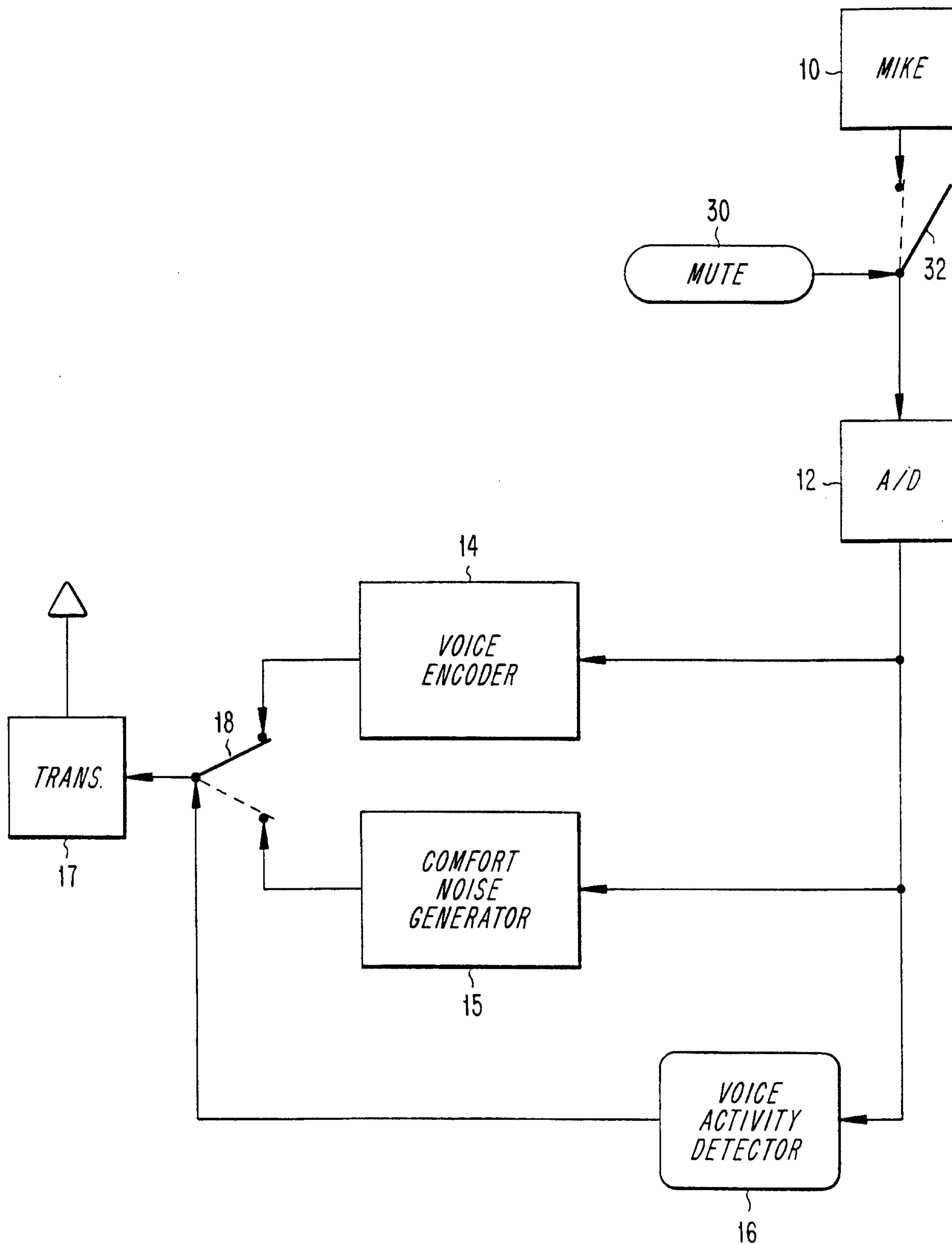
FIG. 3 (PRIOR ART)
