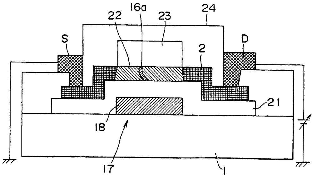
FIG. 14 PRIOR ART
