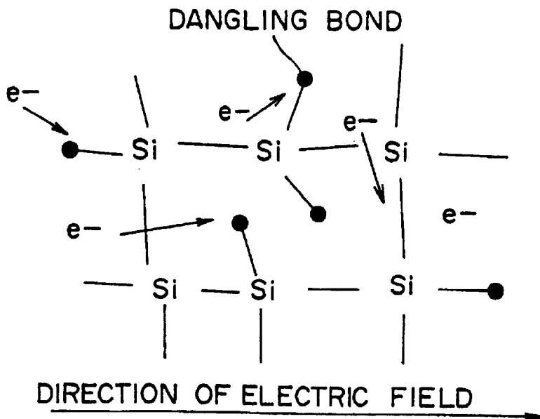
FIG. 16 PRIOR ART
