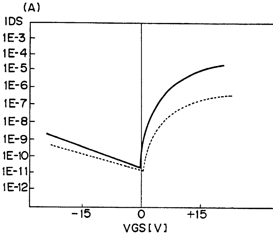
FIG. 15 PRIOR ART
