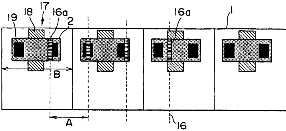
FIG. 13 PRIOR ART
