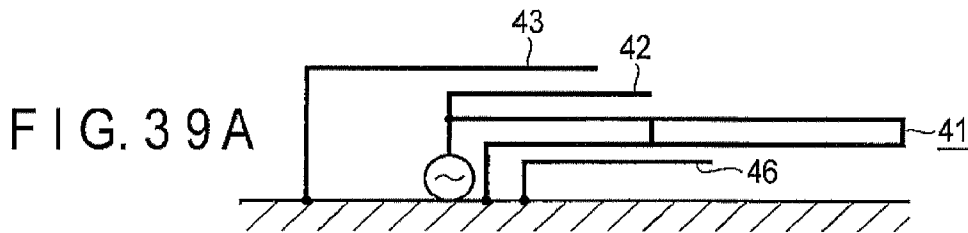
When parasitic element is added on ground terminal side of folded monopole element
