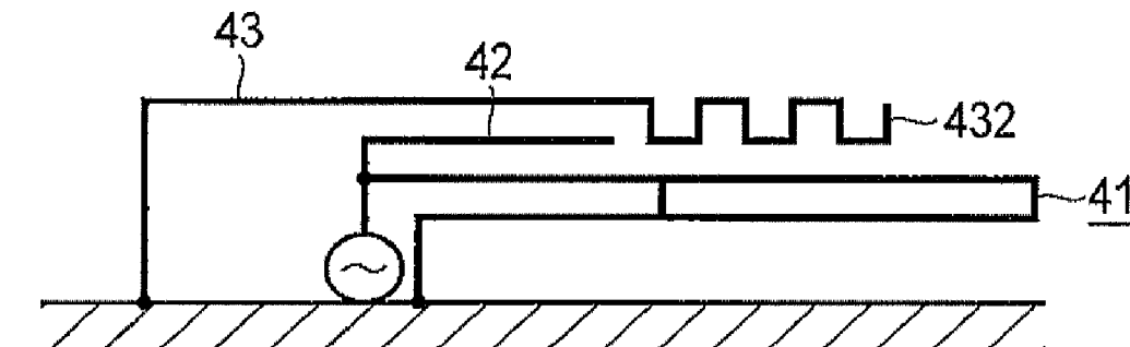
When distal end portion is formed into meandering shape
